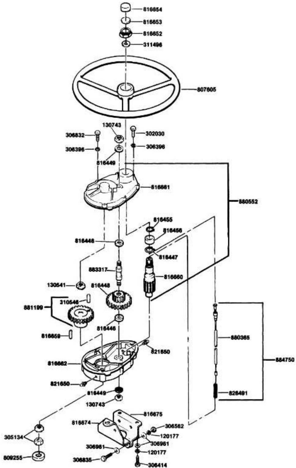
Figure 1: Steering Gear, Horn Button & Wire Assy 7810, 7930 & Later.
